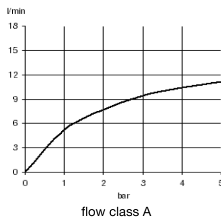
Flow rate diagram
