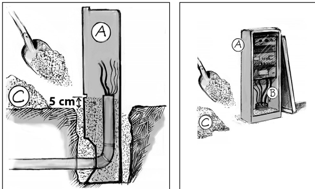
A-Empty housing; B-Seal; C - Dry white sand
