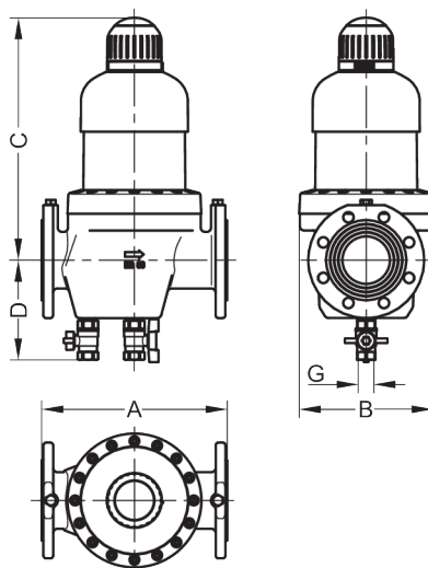
Abb. 7: JPF-QC DN 65 - 100
