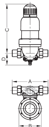
Abb. 6: JPF-QC 1 1/2" - 2"
