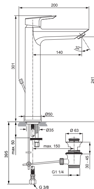
Basin mixer CH3 Vessel with flex. hose with pop-up waste chrome A6574AA
