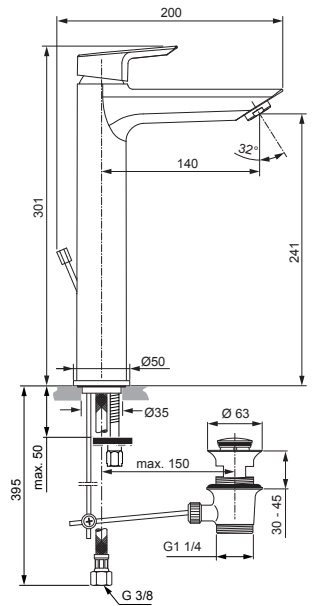
Basin mixer CH3 Vessel with flex. hose with pop-up waste chrome A6574AA
