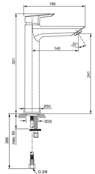
Basin mixer CH3 Vessel with flex. hose without pop-up waste chrome A6576AA
