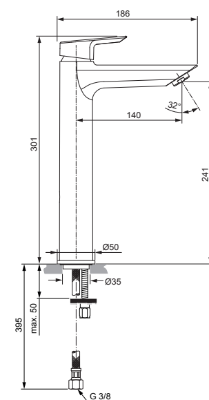
Basin mixer CH3 Vessel with flex. hose without pop-up waste chrome A6576AA
