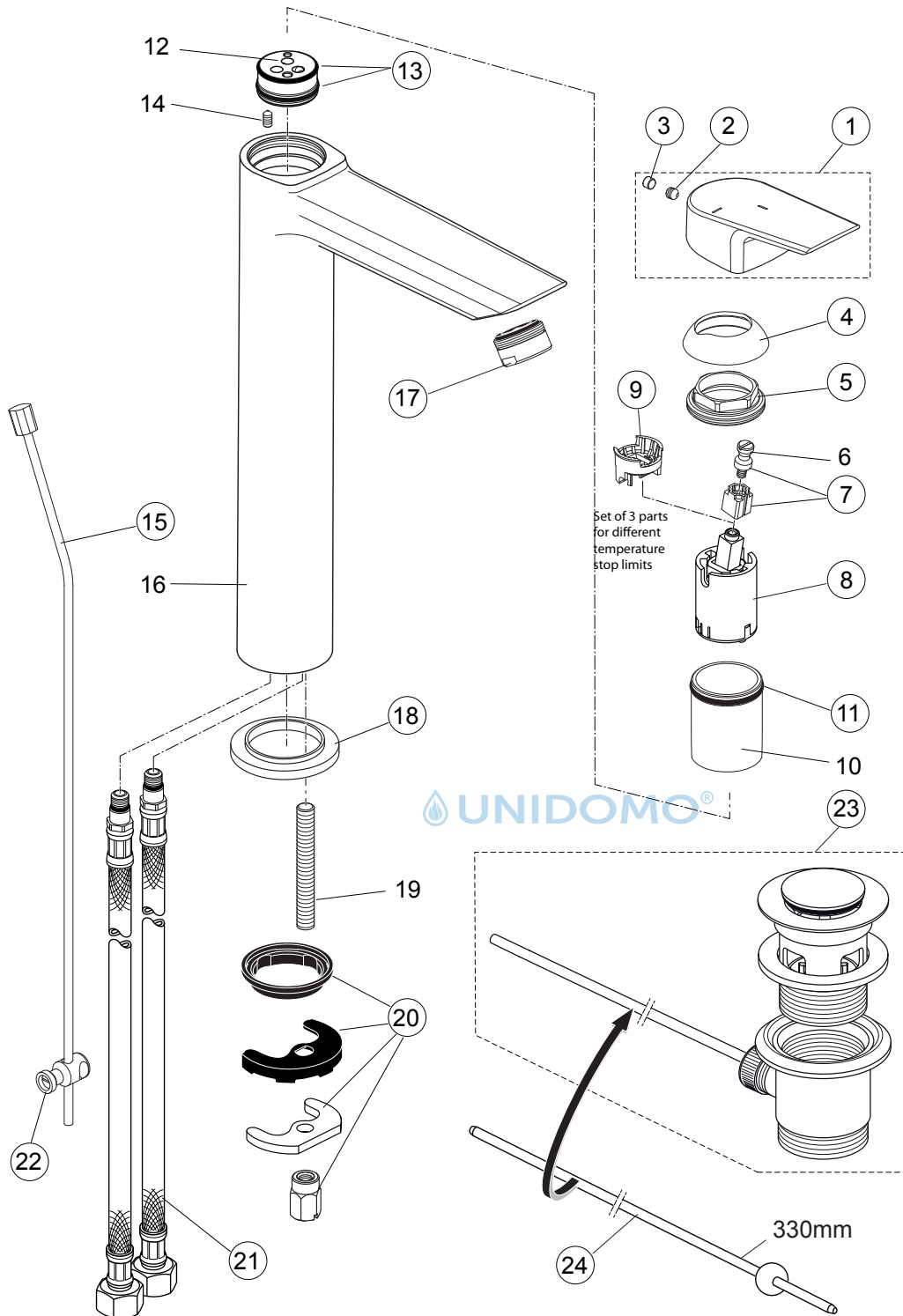
Basin mixer CH3 Vessel with flex. hose with pop-up waste chrome A6574AA
