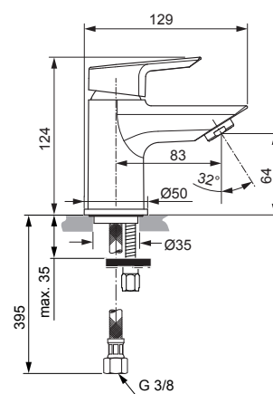
SL basin mixer Piccolo with flex. hose without pop-up waste chrome A6568AA
