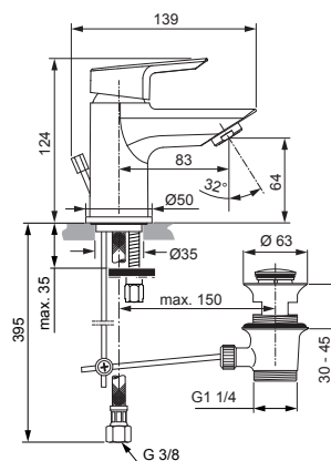
SL basin mixer Piccolo with flex. hose with pop-up waste chrome A6566AA
