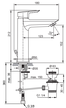
Basin mixer CH3 Grande with flex. hose with pop-up waste chrome A6564AA
