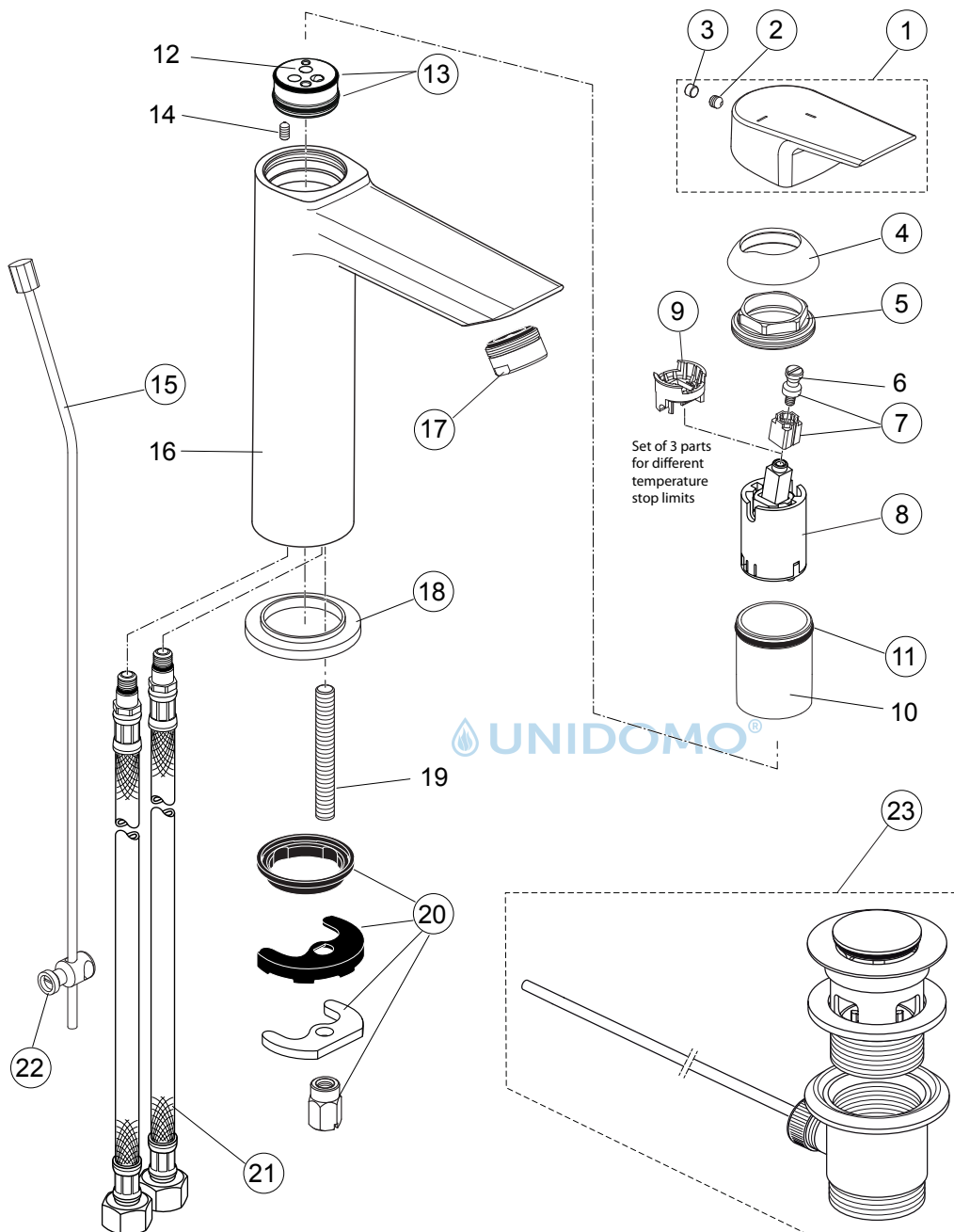
Basin mixer CH3 Grande with flex. hose with pop-up waste chrome A6564AA
