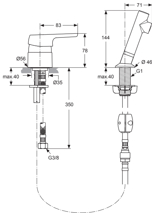
Single Lever hairdresser mixer with pull out hand spray with flex. hoses G3/8 chrome A5727AA
