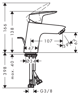
Logis 100 71101000 / 71107000 Logis 100 CoolStart 71103000
