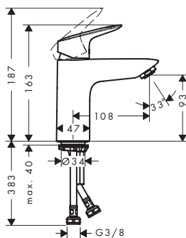
Logis 100 71101000 / 71107000 Logis 100 CoolStart 71103000
