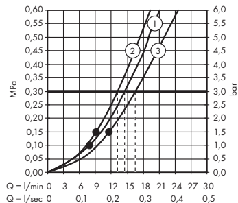
Raindance Select S 150 28587XXX
