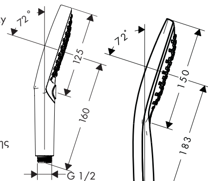
Raindance Select S 150 28587XXX
