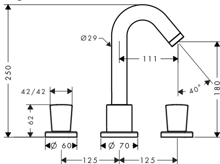
Logis 71300000
