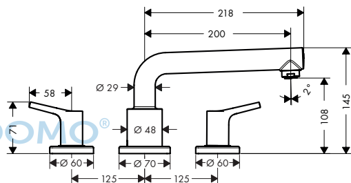
Talis S 72415000
