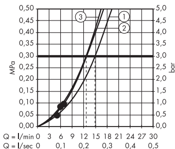
Crometta 85 Multi 28425000
