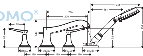
Metropol 32552000
