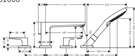
Metropol 74552000
