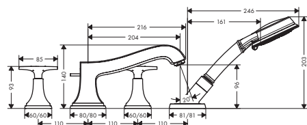
Metropol 74552000
