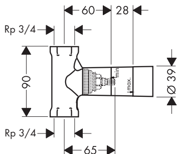
DN20 (3/4") 15970180
