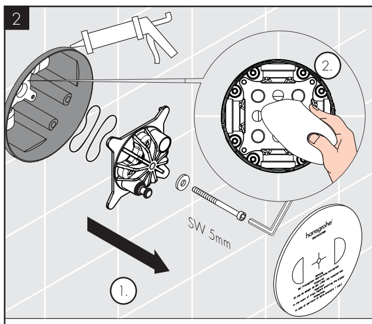
iBox universal 01700180
