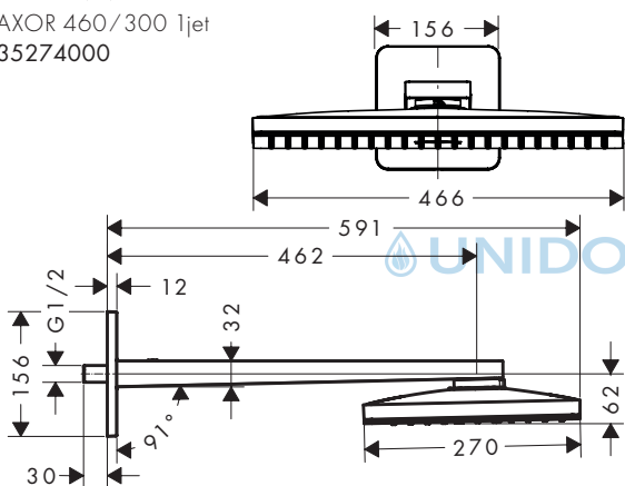
AXOR 460/300 1jet 35278000/35274000
