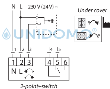
Direct/Inverse function
