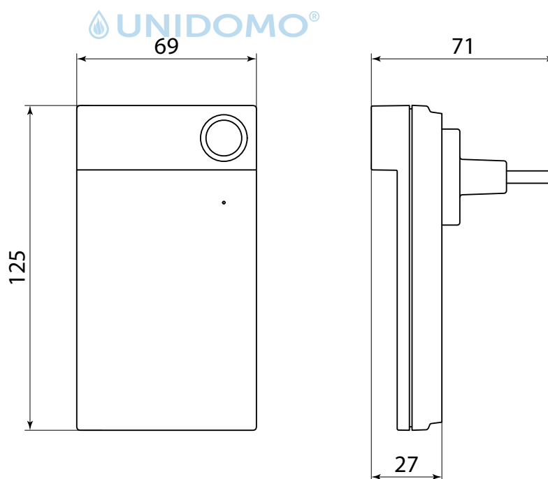
Repeater Modul Danfoss Icon™ 088U1102
