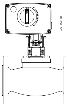
AME 25, AME 35 + VFS-2-Ventile (DN 15–50)
