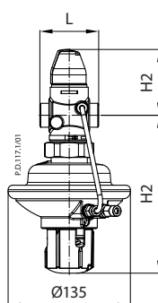
AVPQ DN 15-50 \Delta p = 0,2-1,0 \text{ bar}
