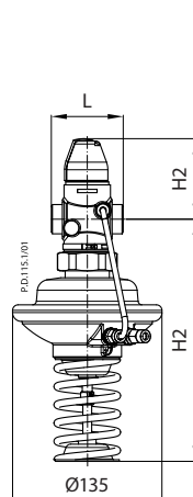
AVPQ DN 15-50 \Delta p = 0,3-2,0 \text{ bar}
