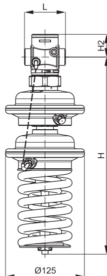
DN 15 - 50 \Delta p = 3 - 11 \text{ bar}
