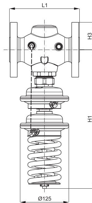
DN 32 - 50 \Delta p = 3 - 11 \text{ bar}
