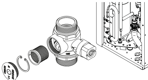
Abb. 14: Demontage Kugelhahn
