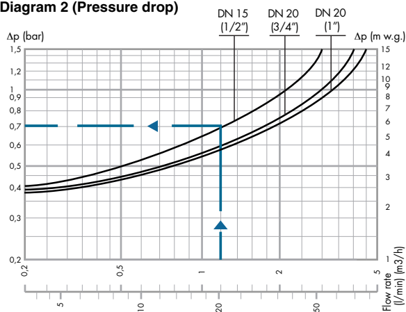
Diagram 2 (Pressure drop)
