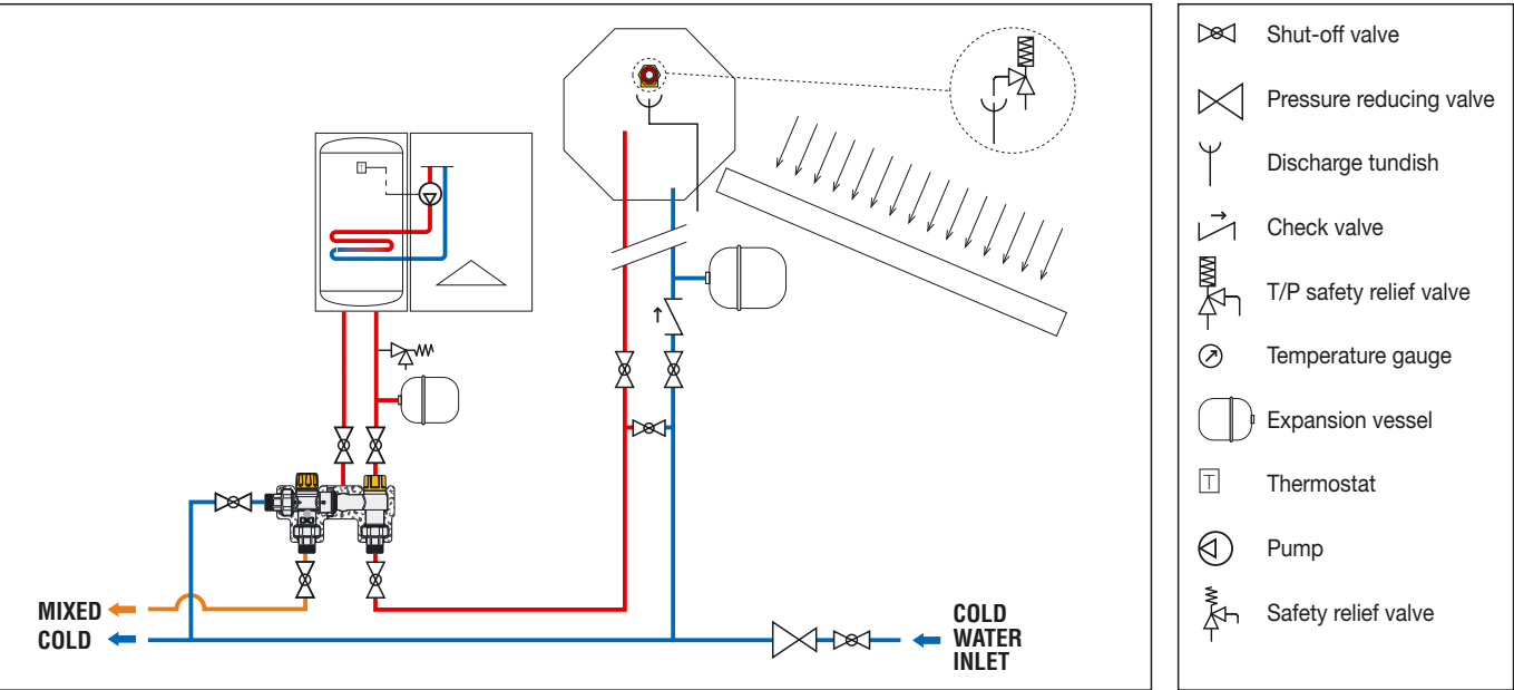
262 series Thermostatic Solarincal - natural circulation solar system
