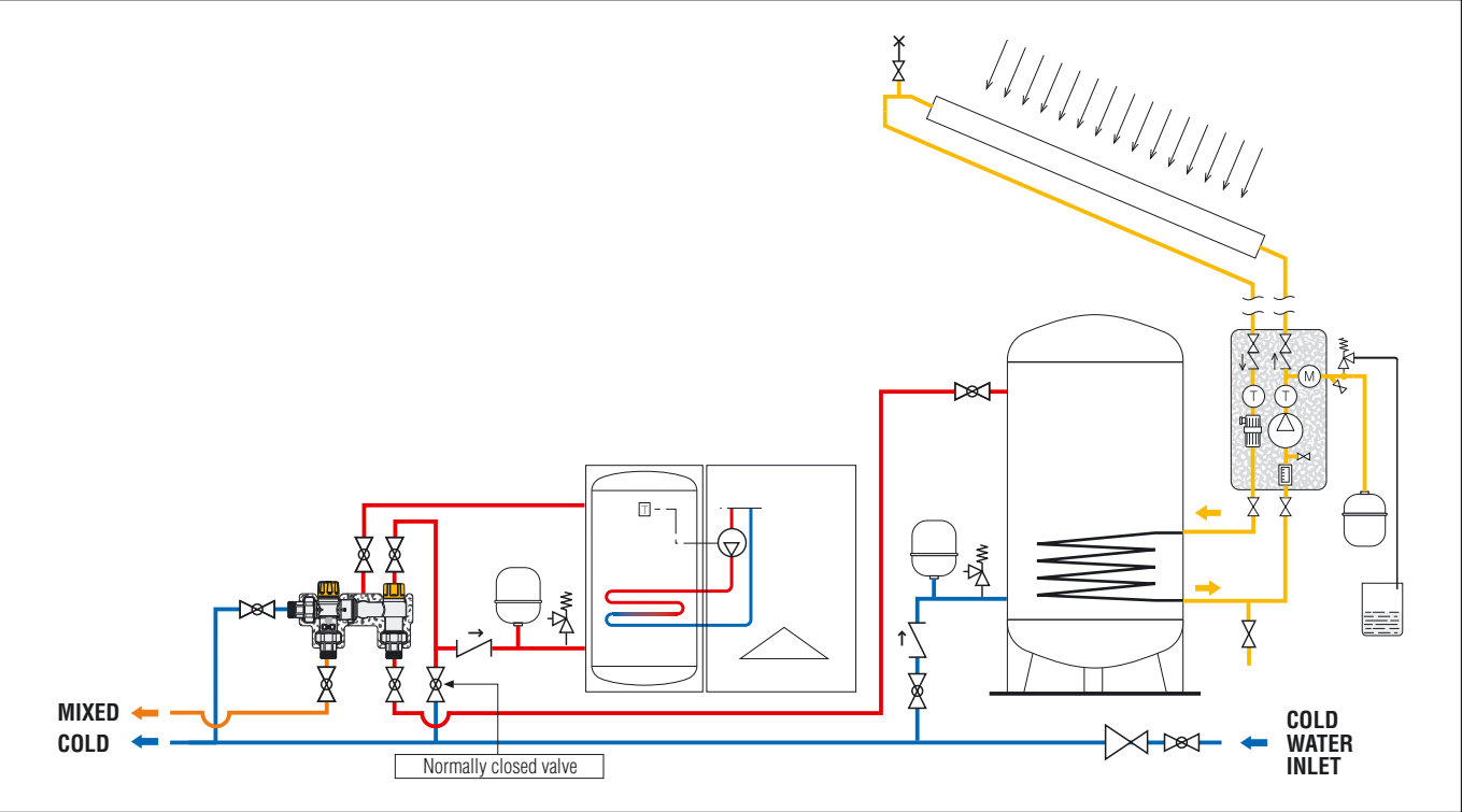
262 series Thermostatic Solarincal - forced circulation solar system
