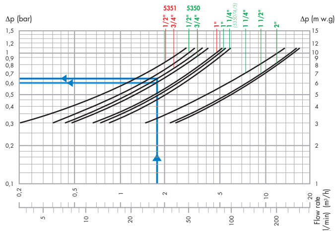
Graph 2 (Pressure drop)
