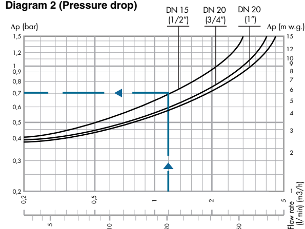
Diagram 2 (Pressure drop)
