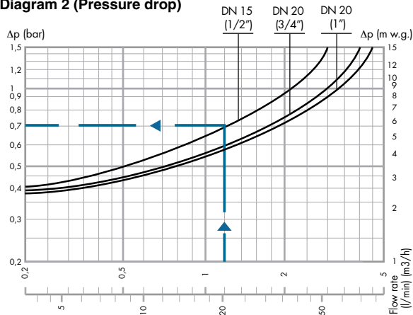
Diagram 2 (Pressure drop)
