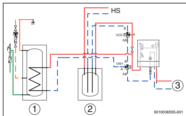
Bild 26 Puffer, VCO-Bypassventil
