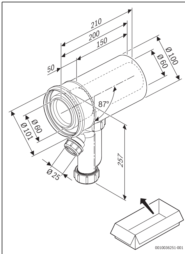
1 Ø60: 7738113563
