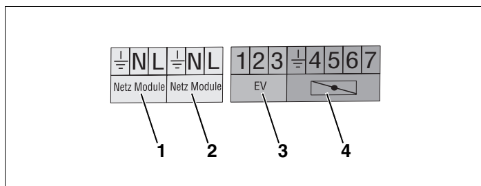
Abb. 2 Anschlüsse 230 V
