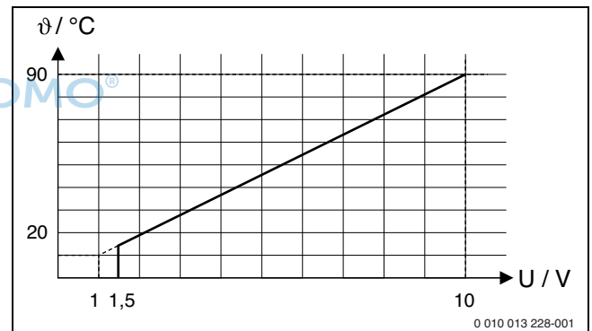
Fig. 2 Linear relationship between the 0–10 V signal ( U in volts) and the demanded flow temperature \theta (in °C with reference to the minimum flow temperature range to the maximum flow temperature range [default setting 20 °C to 90 °C])
