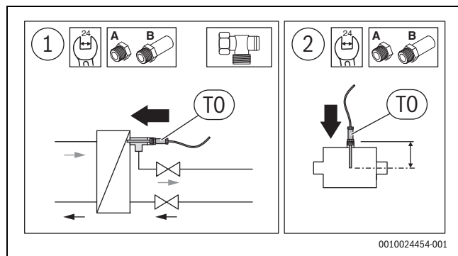
Fig. 3 Optimised sensor installation
