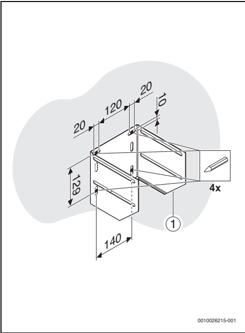
6 Ø 125: 7738112710/...711/...712
