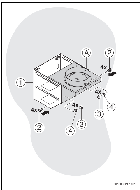
9 Ø 125: 7738112710, Ø 160: 7738113153
