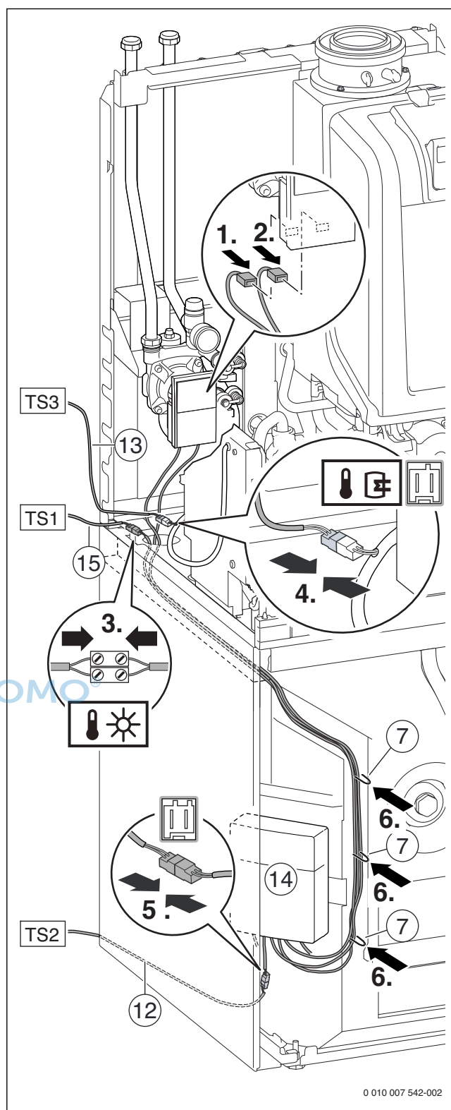
17 GC9000iWM..100..
