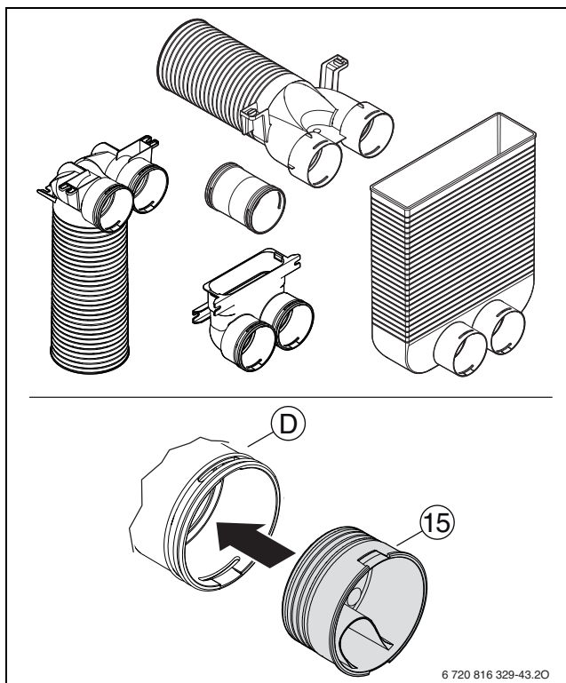
Fig. 89 RR 75... + RRS 75
