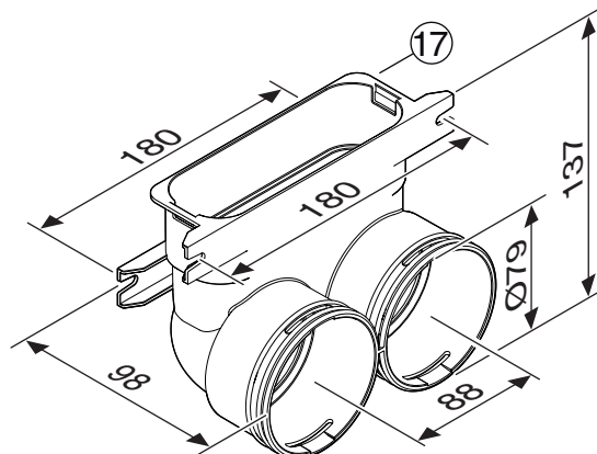
Fig. 18 RRB 75
