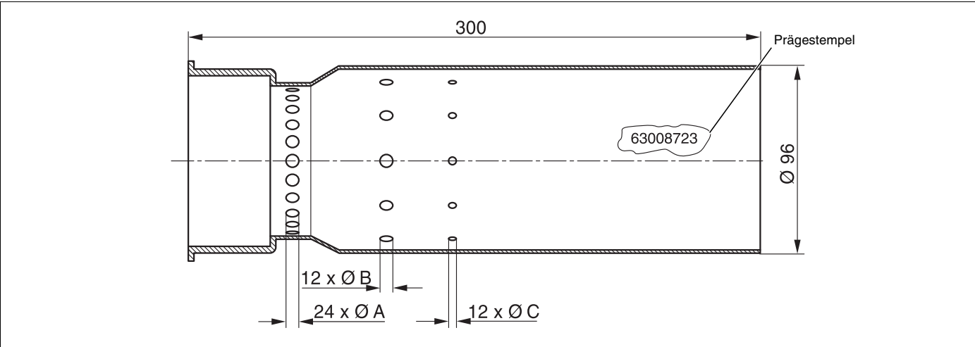
Abb. 9 Brennerrohr BE-A2.0 – 68
