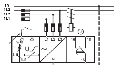
Circuit diagram for the new phase guard
