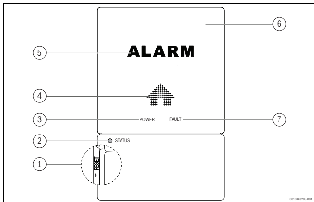
Fig. 1 Product overview
