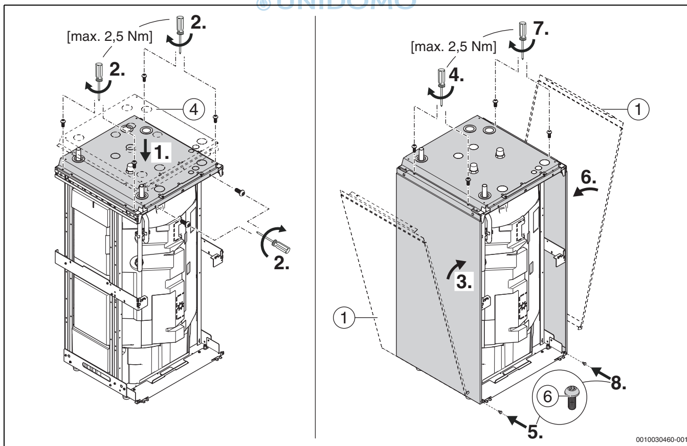
12 SWDP 200/SCDP 250
