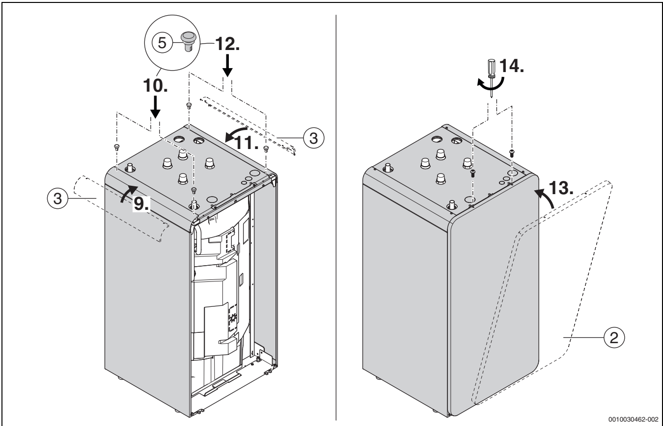
13 SWDP 200/SCDP 250
