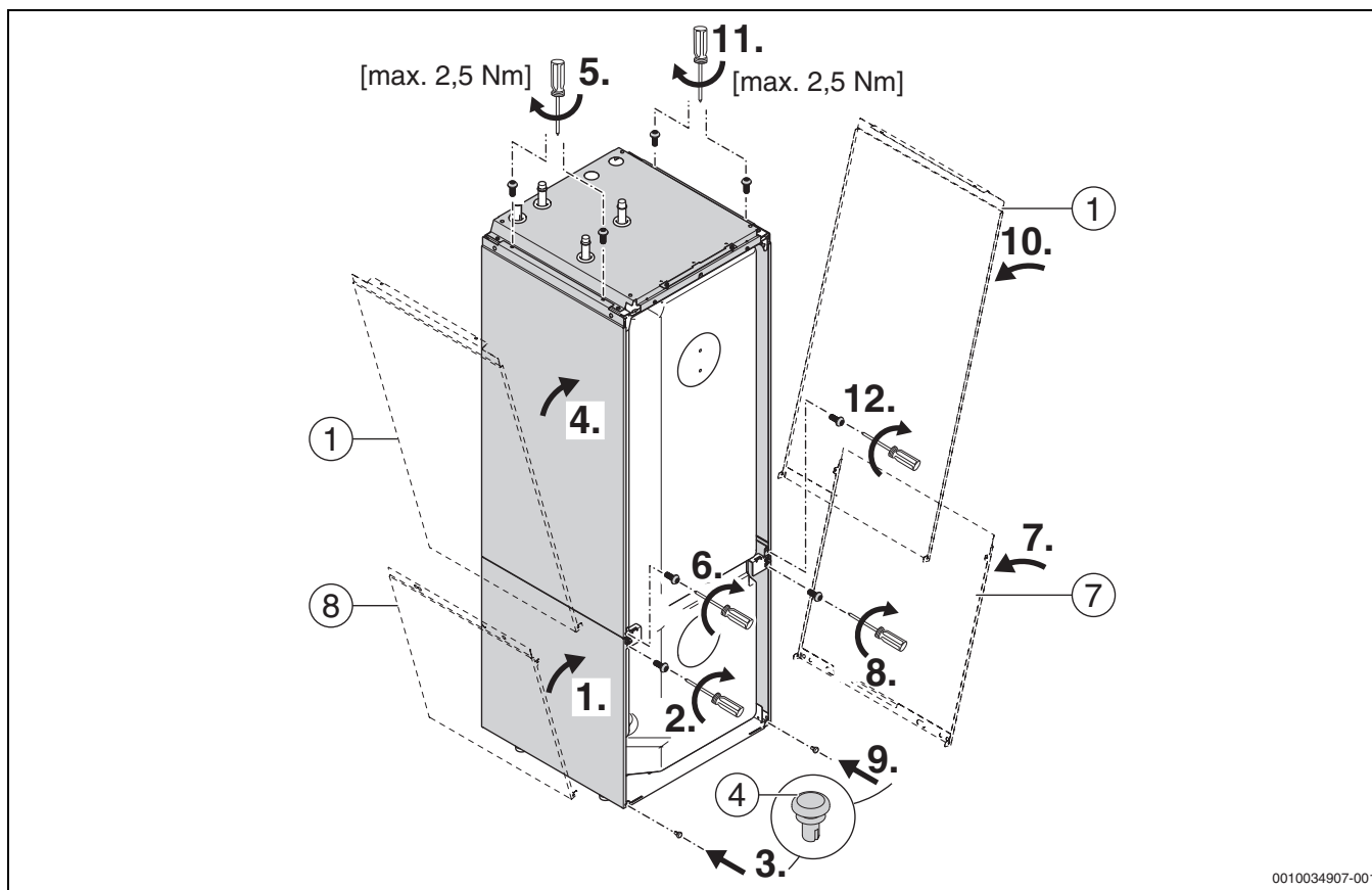
15 SWDP 300/SWDPS 300
