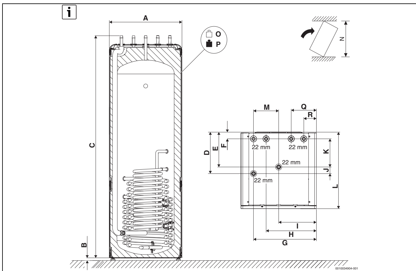
6 SWDPS 300
