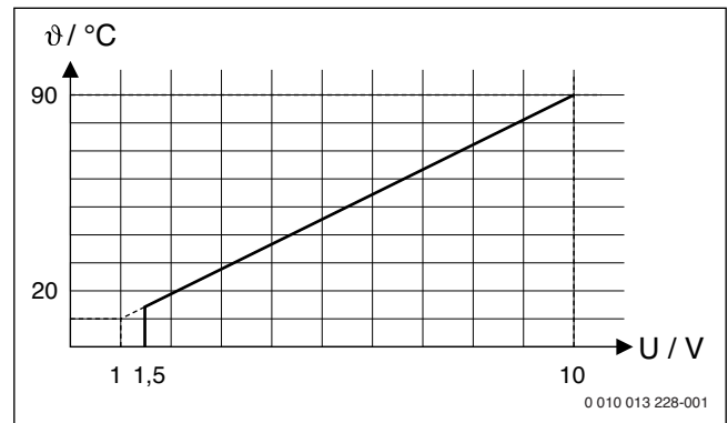
Fig. 9 Linear relationship between the 0-10 V signal (U in volts) and the demanded flow temperature \Theta (in °C with reference to the minimum flow temperature range to the maximum flow temperature range [default setting 20 °C to 90 °C])
