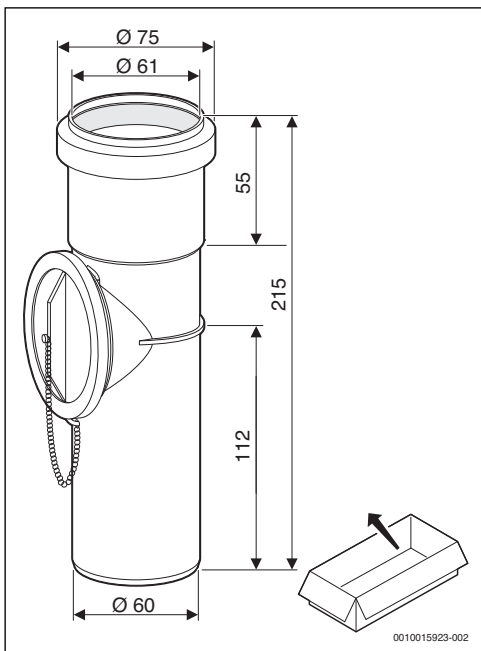
1 FC-SR60: 7738112630
