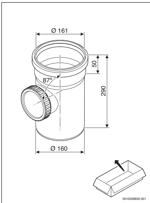
5 FC-SR160: 7738113121
