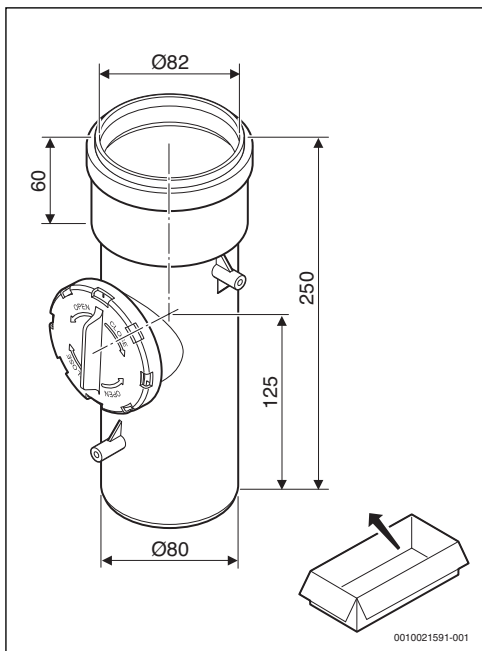
2 FC-SR80: 7738112669
