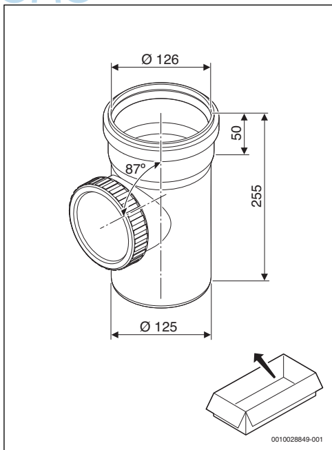
4 FC-SR125: 7738113114
