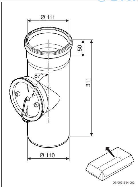
3 FC-SR110: 7738112684
