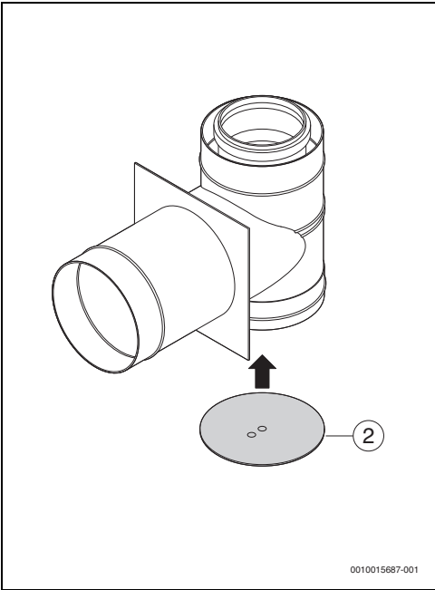
9 C_{53x} FC-C125: 7738112490
