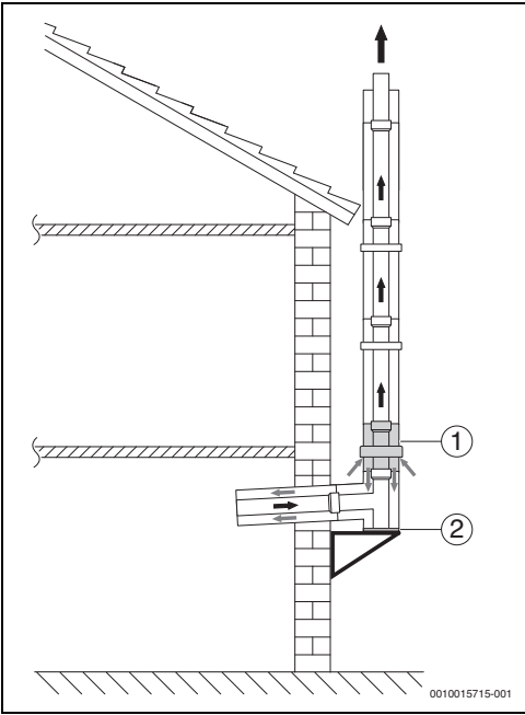
7 C_{53x} FC-C125: 7738112490
