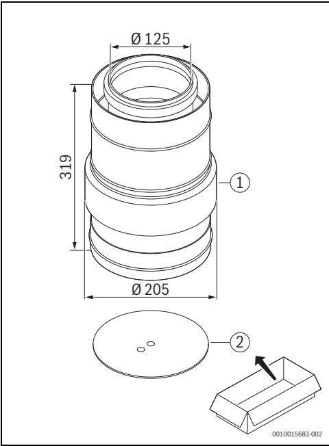
1 FC-C125: 7738112490
