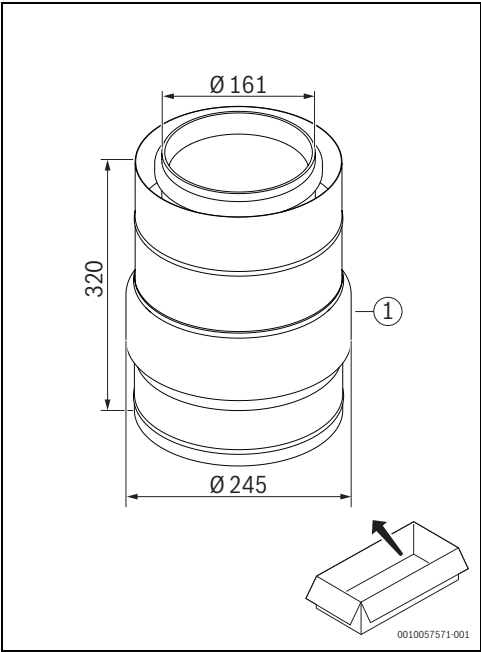
2 FC-C160: 7738114040
