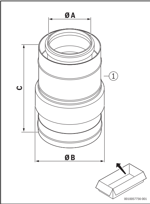
3 FC-C200: 7738112491, FC-C250: 7738112492
