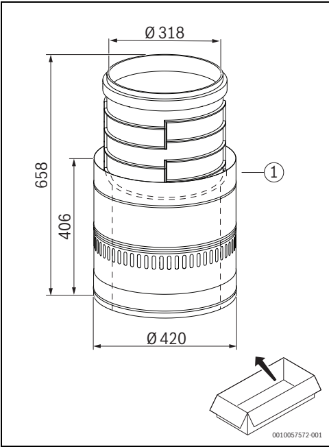
4 FC-C315: 7738114041
