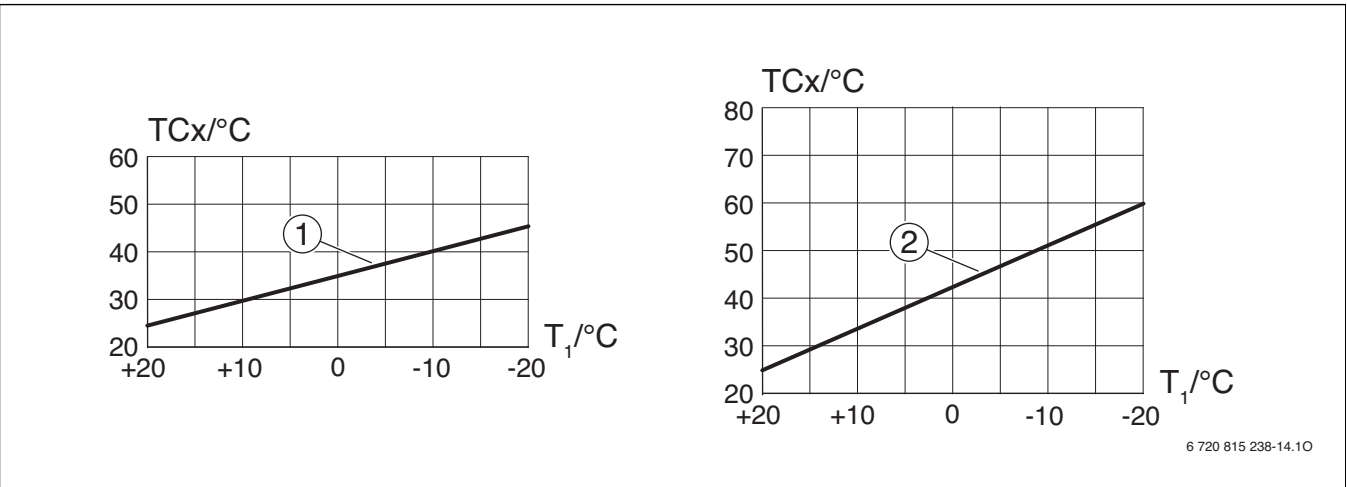
Bild 10 Setting of simple heating curve
