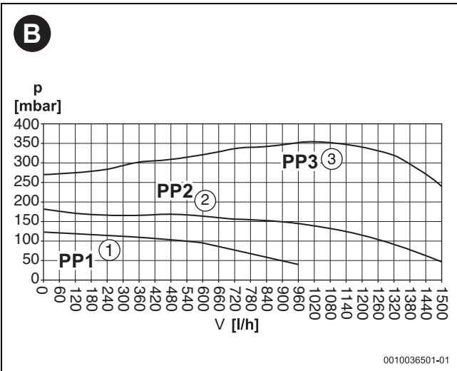
3 de: Restförderhöhe (Proportionaldruck-Kennlinie) / en: residual head (proportional pressure curve)
