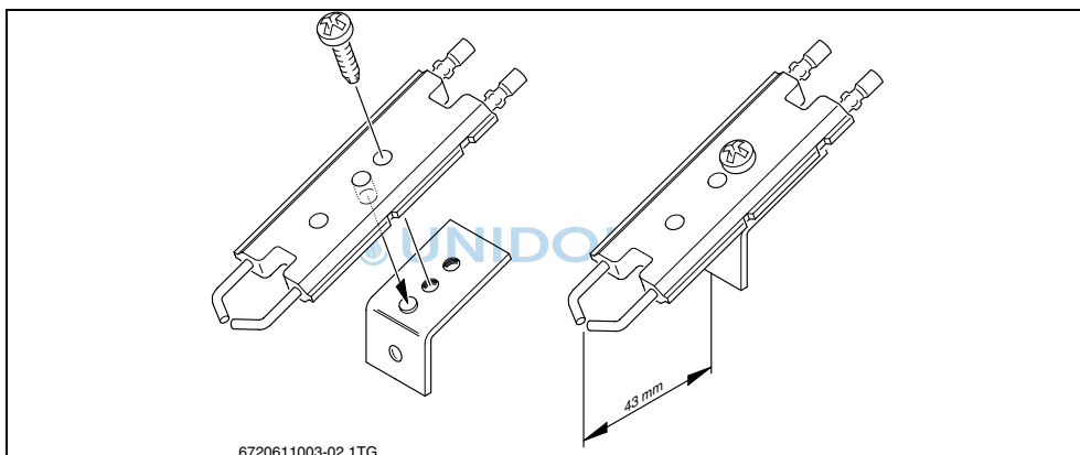
2 KS/KSN 12...42-7 E
