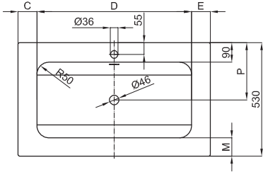
BetteOne 900 x 530 mm
