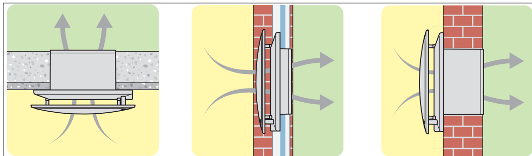
Abb 173: Montage Abluftventilator VAE 90 AHT
