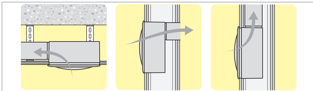
Abb 174: Montage Abluftventilator VAE 190 RHT
