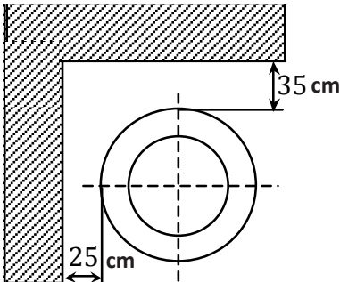
Illustration: Distances from walls
