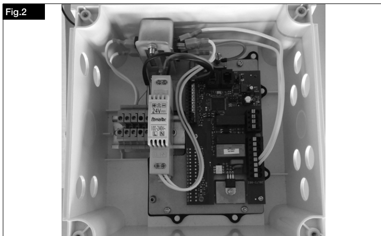
4.2 Connection of the control board
