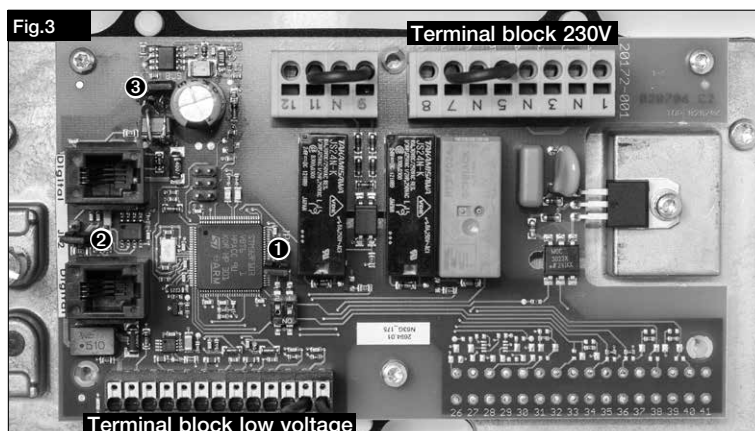
4.2 Connection of the control board
