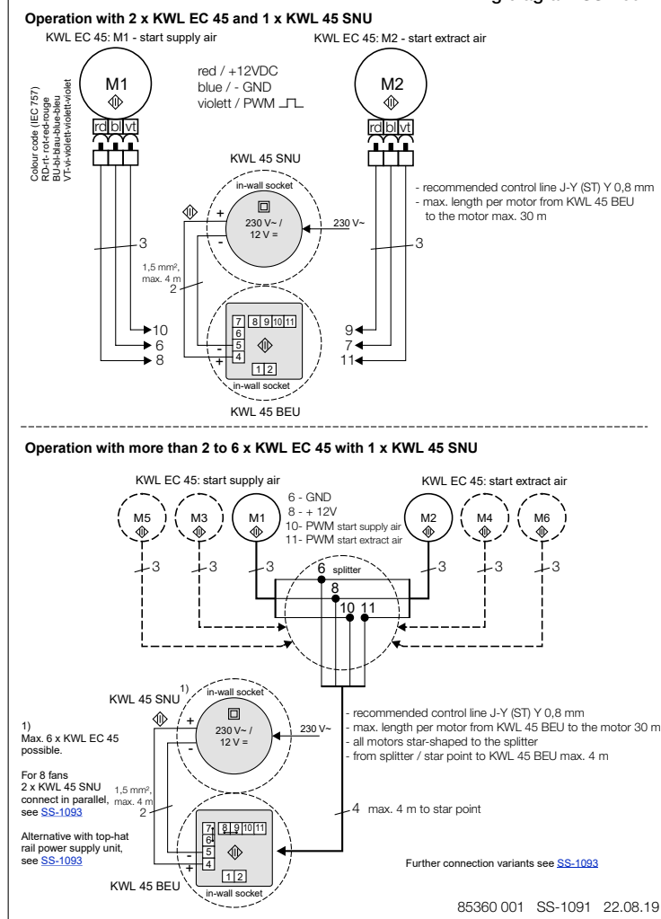
Wiring diagram SS-1091
