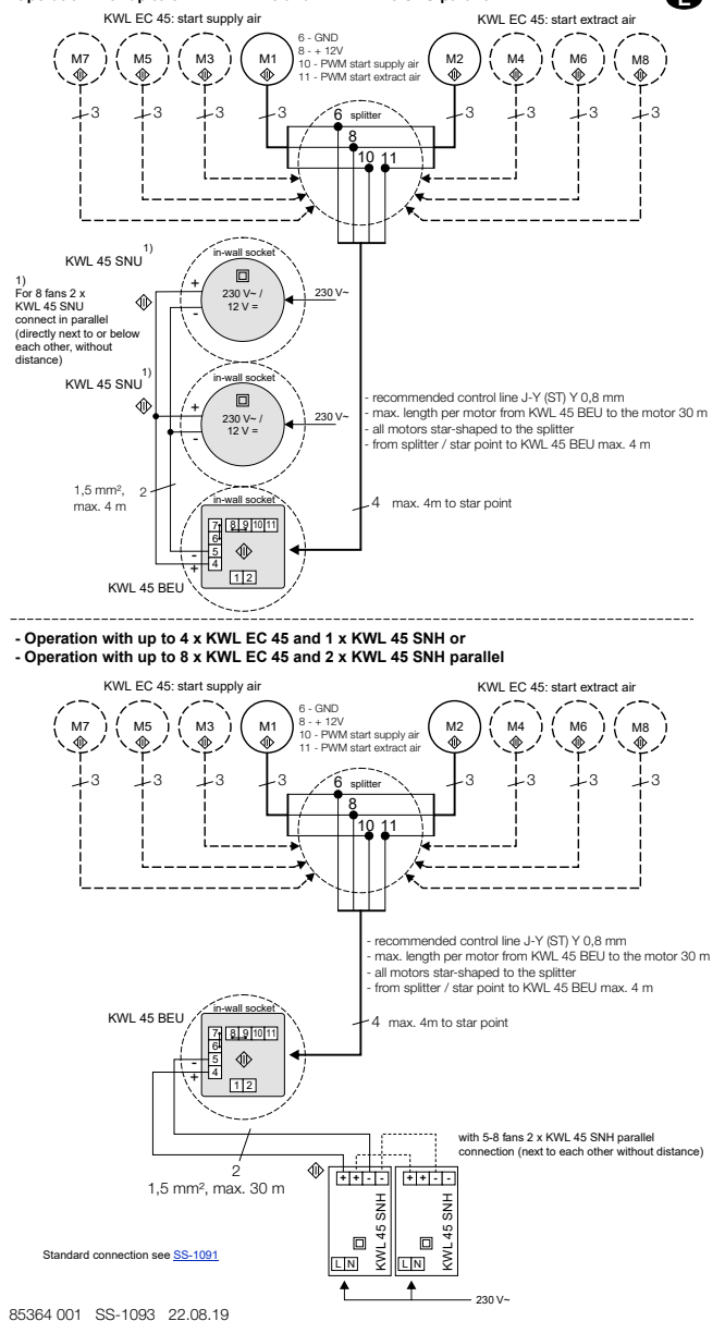
Wiring diagram SS-1093
