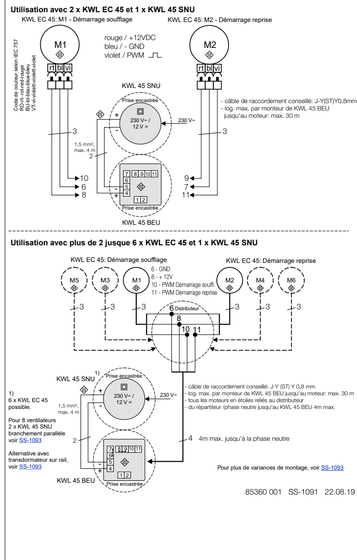
Plan de raccordement SS-1091
