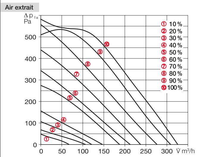
Characteristic curve KWL 300 W ET
