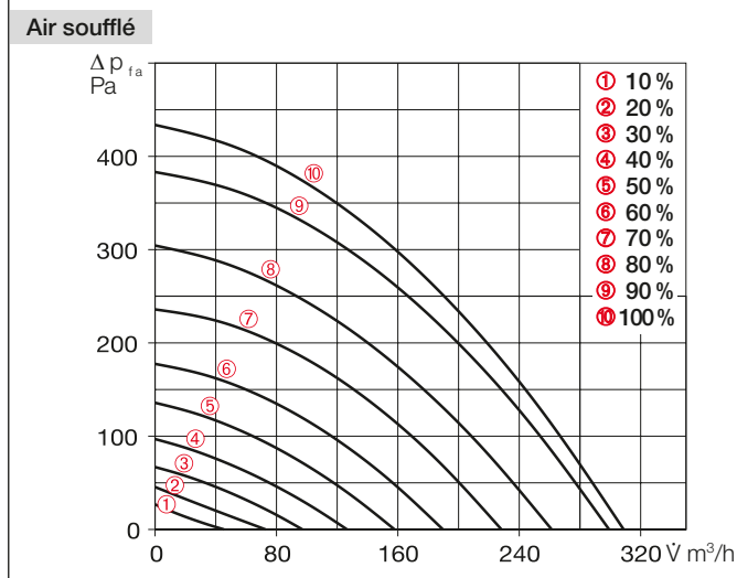
Characteristic curve KWL 300 W
