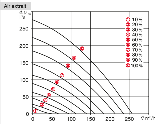
Characteristic curve KWL 200 W ET
